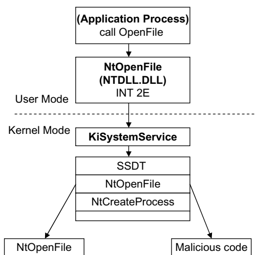
Fig. 14.4. System Service Dispatch Table. Upon invocation of the OpenFile API, execution flows from the user mode function in located in KERNEL32.DLL to the interface in NTDLL.DLL . NTDLL generates the system call interrupt that causes a transition to kernel mode. The interrupt handler, KiSystemService , looks up the requested function address in the System Service Descriptor Table (SSDT) and calls it. A rootkit may replace the address in the SSDT to globally intercept Operating System services.
