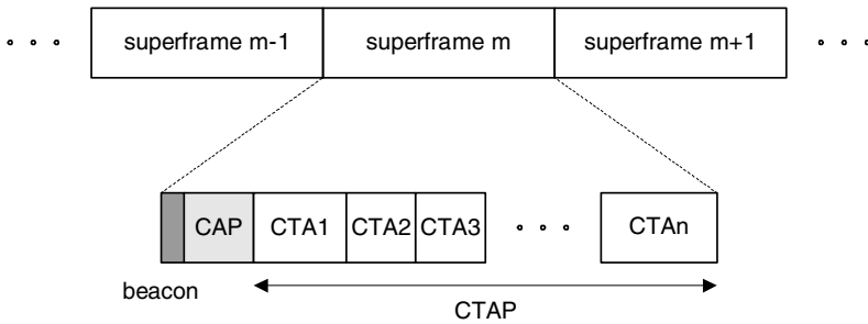
Fig. 16.1. Superframe structure in an 802.15.3 network.
