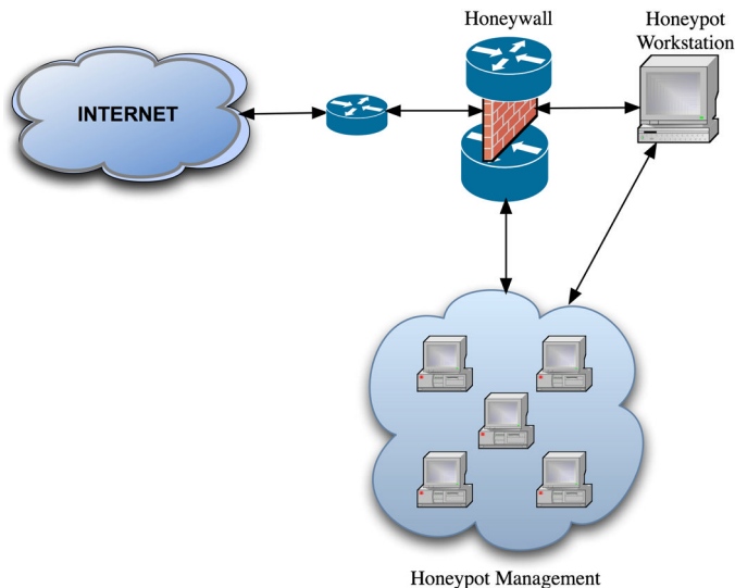
Fig. 15.8. Honeypot (Honeynet) Diagram.
