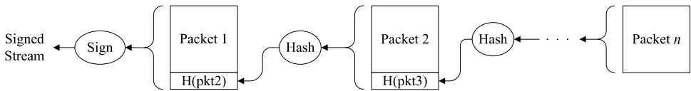
Fig. 4.2. Stream authentication using hash chaining.
