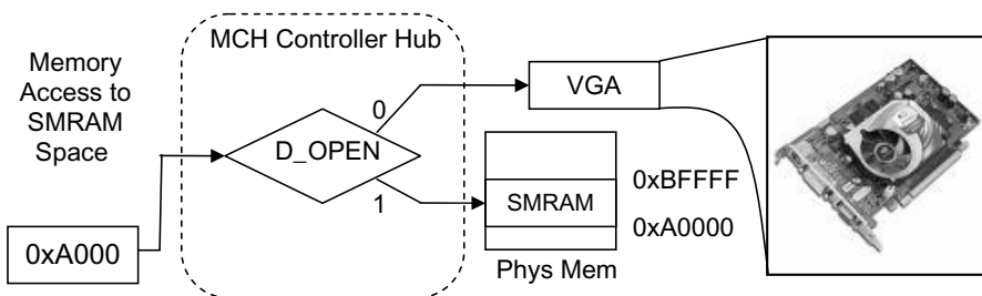
Fig. 14.7. SMRAM memory accesses are filtered by the chipset based upon their origin and the state of the ‘open’ bit in the SMRAM control register. SMM accesses are normally directed to SMRAM while non-SMM accesses are directed to VGA memory.
