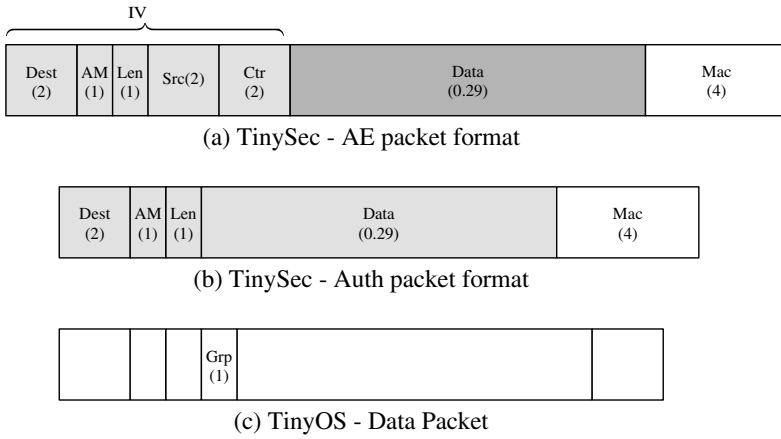
Fig. 21.1. TinySec Data Packet (Legends: Dest : Destination address; AM : Active Message type; it is similar to port numbers in TCP/IP. The AM type specifies the appropriate handler function to decrypt, extract and interpret the message on the receiver side; Len : Length).
