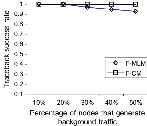
Fig. 6.7. DoS attacker traceback success rate comparison between F-MLM and F-CM.
