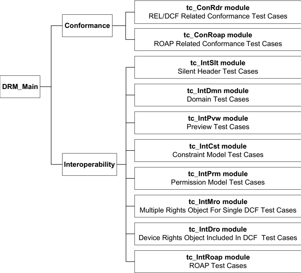
Fig. 19.7. The structure of the DRM ETS.
