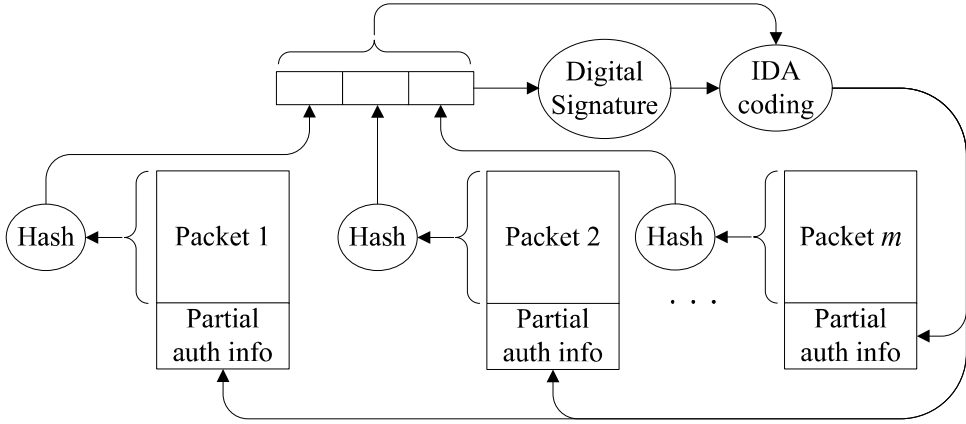
Fig. 4.4. Stream authentication using SAIDA.
