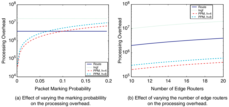
Fig. 7.6. The processing overhead per unit time for filters and probabilistic packet marking (PPM) schemes. Marking scheme has less processing overhead than filtering scheme if the marking probability is not too high (e.g., p \leq 0.07 ).
