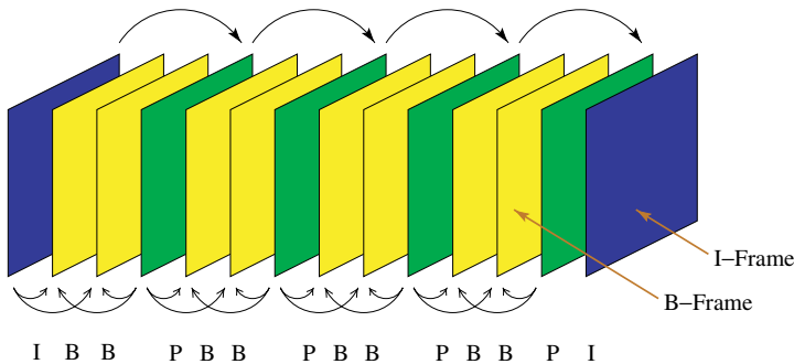
Fig. 4.1. I, P, and B frames in a video sequence.
