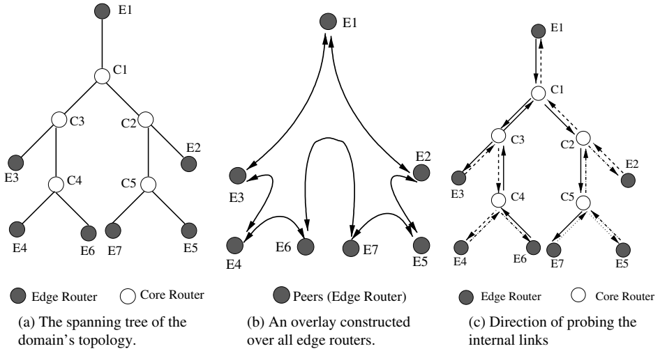
Fig. 7.4. Network monitoring using the distributed mechanism.
