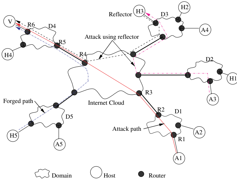
Fig. 7.1. Different scenarios for DoS attacks. Attacker A1 launches an attack on the victim V . A1 spoofs IP address of host H5 from domain D5 . Another attacker A3 uses host H3 as a reflector to attack V .
