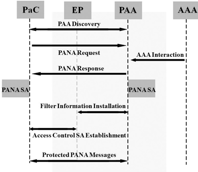
Fig. 1.21. PANA framework.
