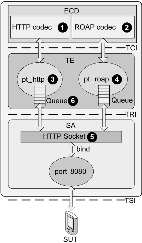
Fig. 19.8. Interaction between the SA and the TE in NTP-DRMT.
