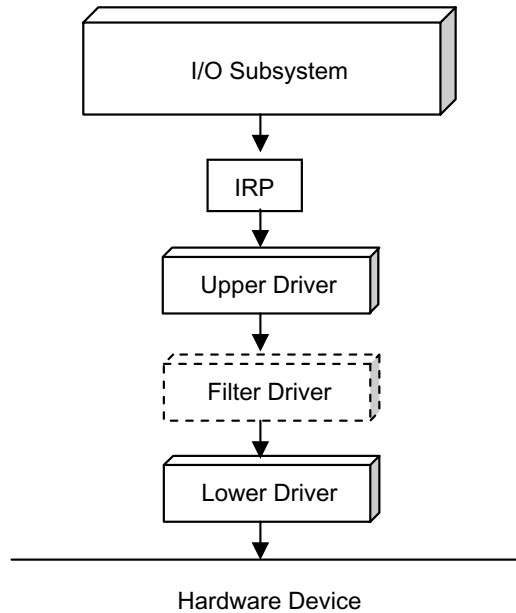
Fig. 14.6. Windows device stack.
