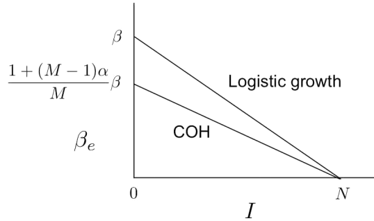
Fig. 12.5. Effective contact rate for COH model and simple homogeneous model.
