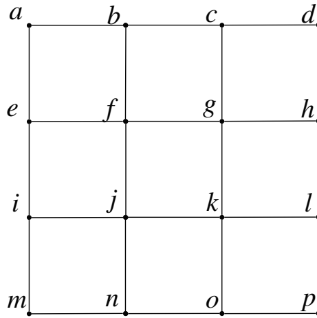
Fig. 18.3. An example 2-connected graph. A = \{a, c, j, l, m, o\} is a DS. B = A \cup \{b, f, i, k\} is a CDS. C = \{a, c, f, h, i, k, n, p\} is a 2-DS. D = C \cup \{b, d, e, l, m, o\} is a 2-CDS.
