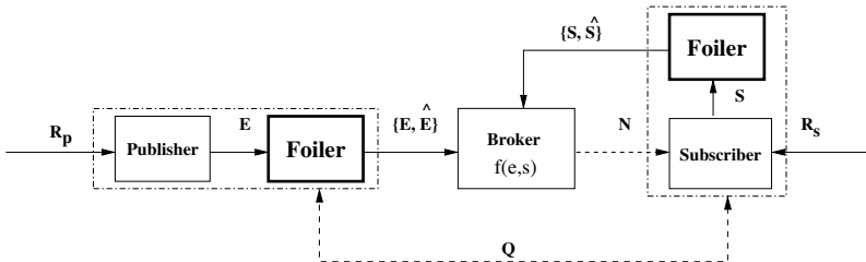
Fig. 2.2. The information foiling mechanism.
