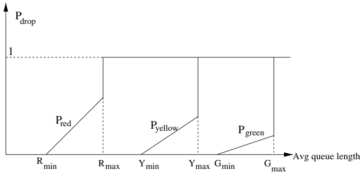
Fig. 7.3. RED Parameters for an active queue with three drop precedences.
