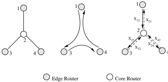
Fig. 7.5. (a) Spanning tree of a simple network topology. (b) Each edge router probes its neighbor edge router in counter-clockwise direction (c) Direction of internal links for each probing.
