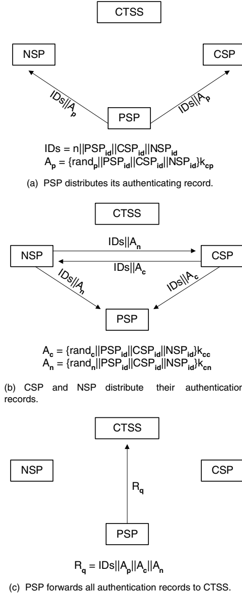
Fig. 20.3. Mutual authentication and session key distribution using keys shared with CTSS.
