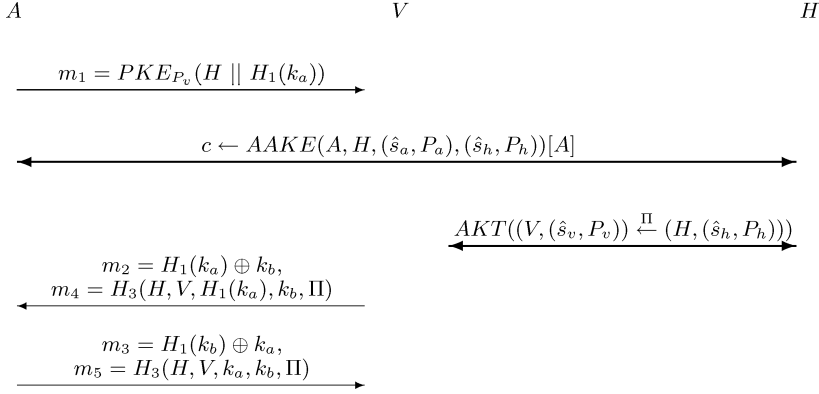
Fig. 8.8. A generic anonymous roaming protocol.
