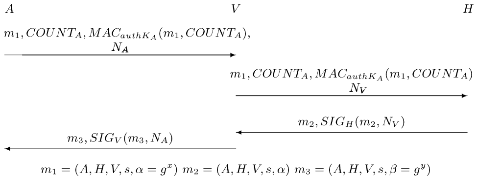
Fig. 8.5. The Yang-Wong-Deng secure roaming protocol.
