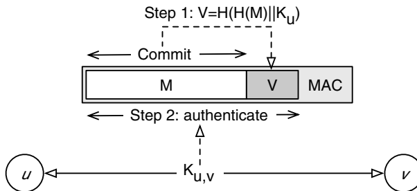
Fig. 9.2. Example packet format in Scheme I.
