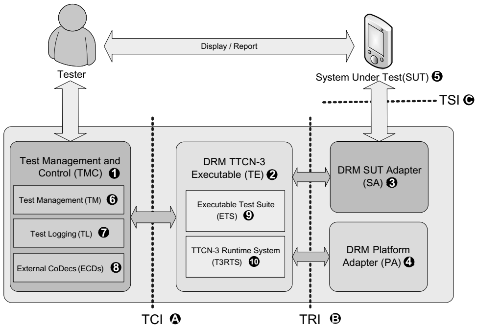
Fig. 19.5. TTCN-3 based NTP-DRMT.
