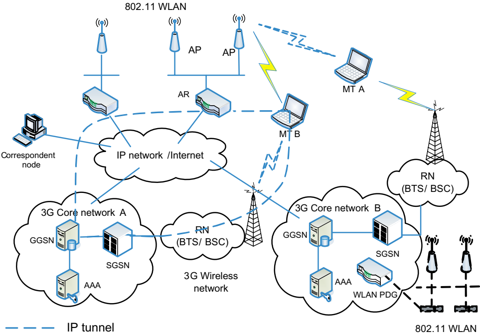
Fig. 17.1. Integrated 802.11 WLAN and 3G cellular networks.
