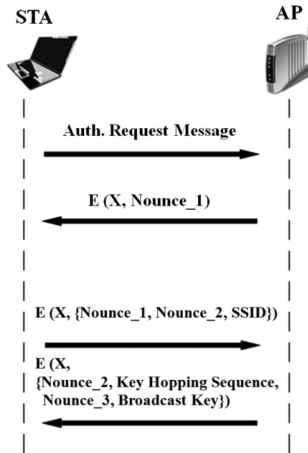
Fig. 1.25. DRKH authentication process.
