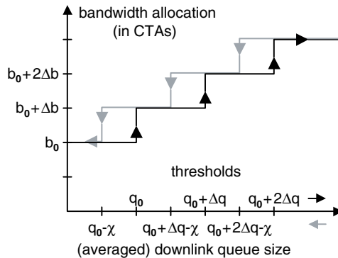
Fig. 16.7. Adaptive CTA allocation with hysteresis.
