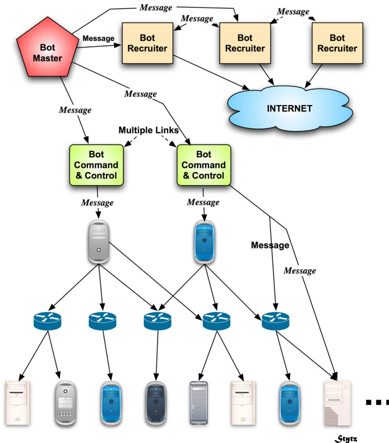
Fig. 15.5. Nominal bot army configuration.
