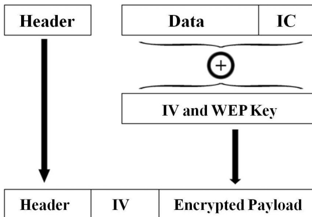
Fig. 1.13. WEP packet encryption.
