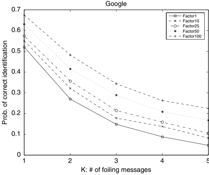
Fig. 2.4. Google data set: Indistinguishability
