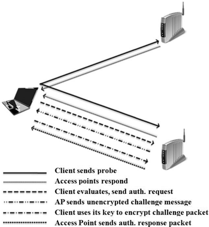
Fig. 1.12. Shared key authentication.
