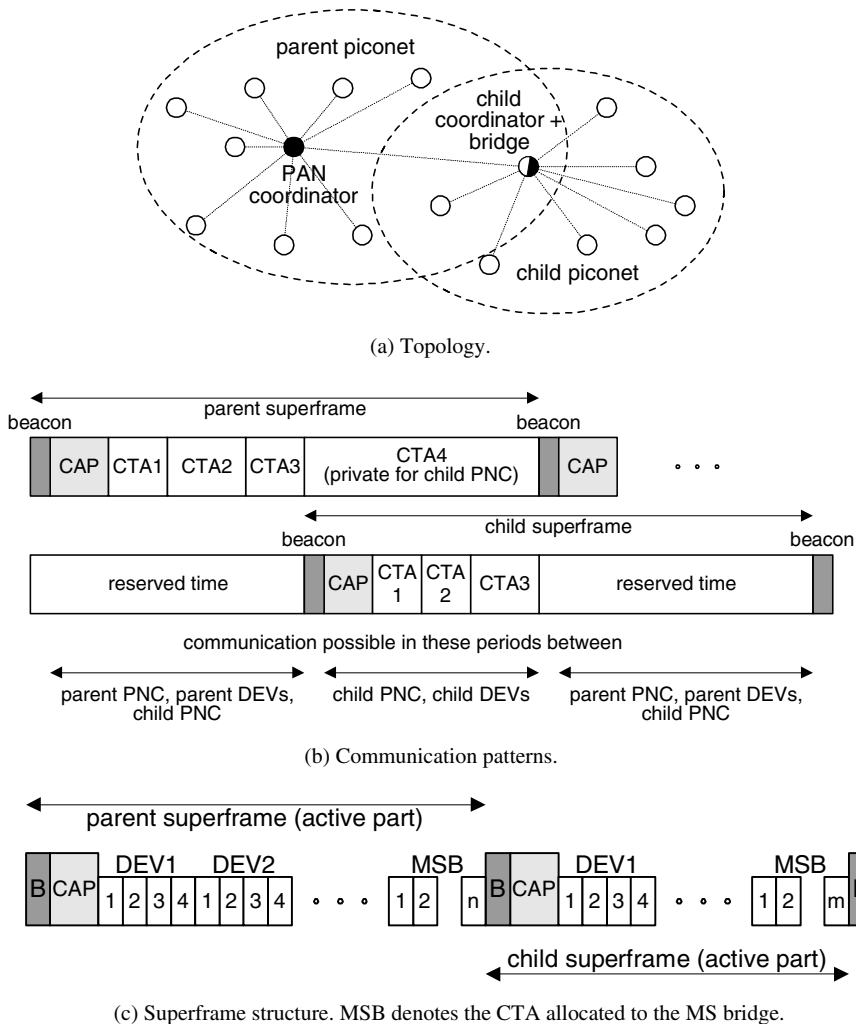
Fig. 16.2. Parent-child interconnection.
