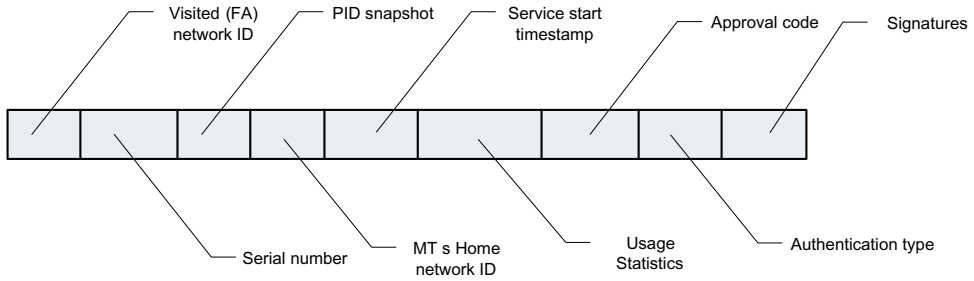
Fig. 17.7. Event ID data structure.
