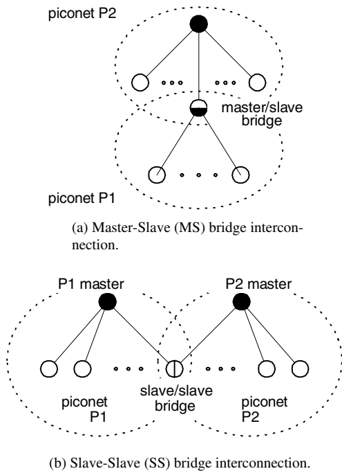
Fig. 16.3. Bridge topologies for multi-piconet networks.
