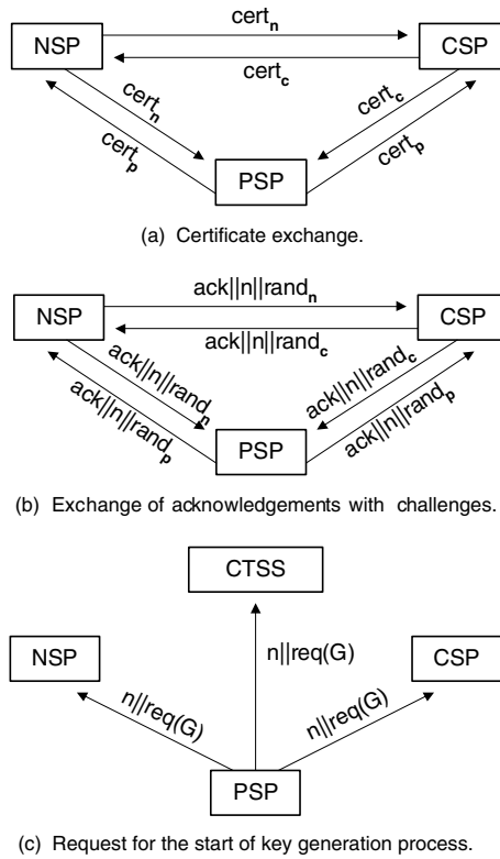
Fig. 20.5. Mutual authentication using ECC certificates.
