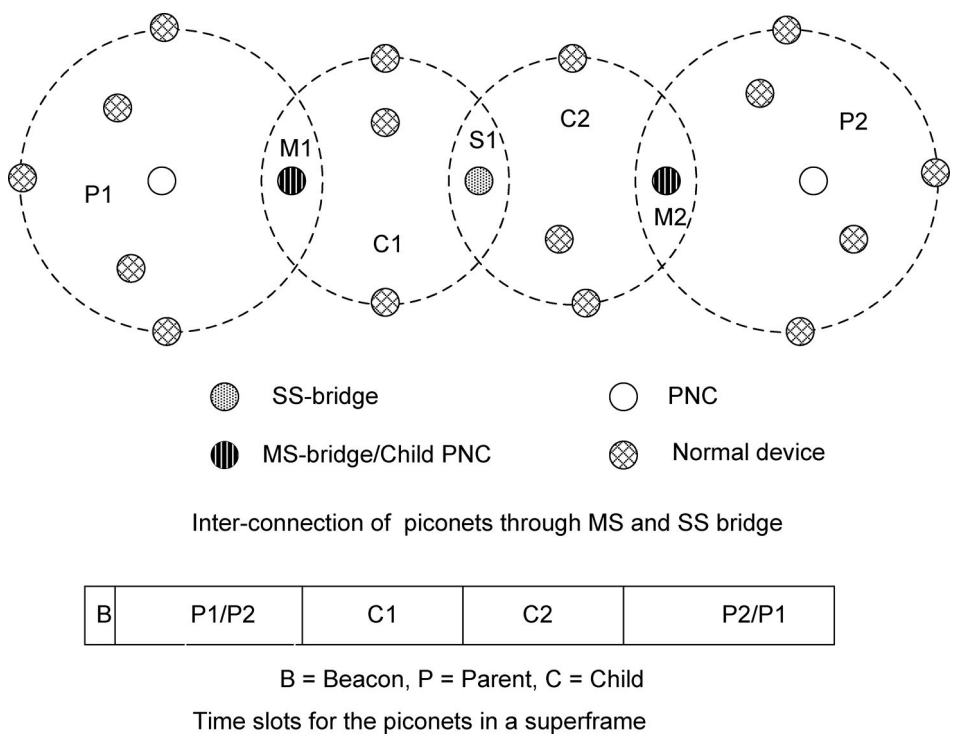
Fig. 16.4. A multi-piconet structure that employs both types of bridge interconnection.
