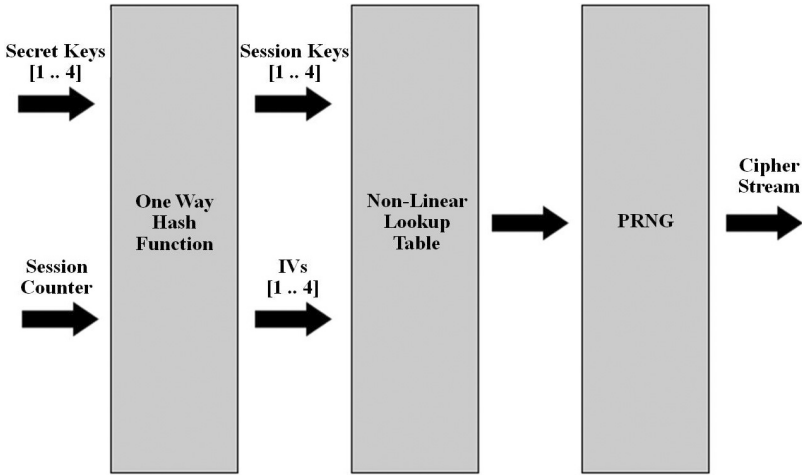
Fig. 1.24. Schematic diagram of DRKH protocol.
