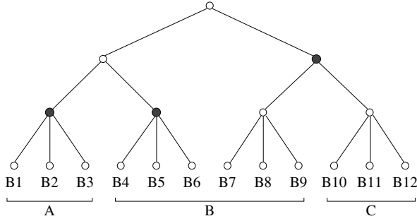
Fig. 4.5. Stream authentication using TFDP [31].
