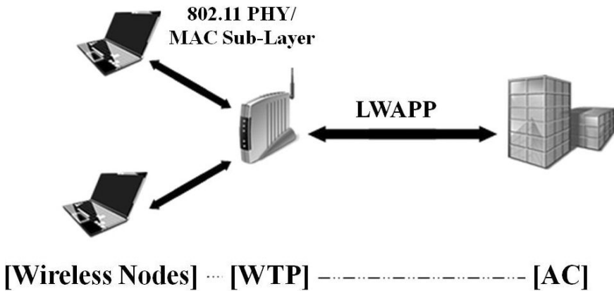
Fig. 1.22. LWAPP architecture.
