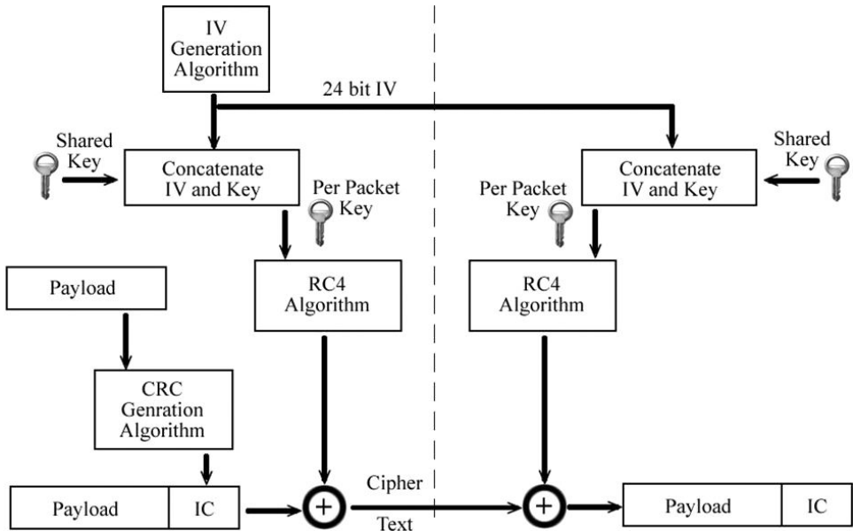
Fig. 1.14. WEP encryption and decryption processes.
