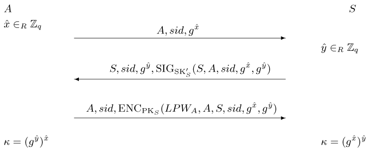
Fig. 8.1. A password AKE protocol.
